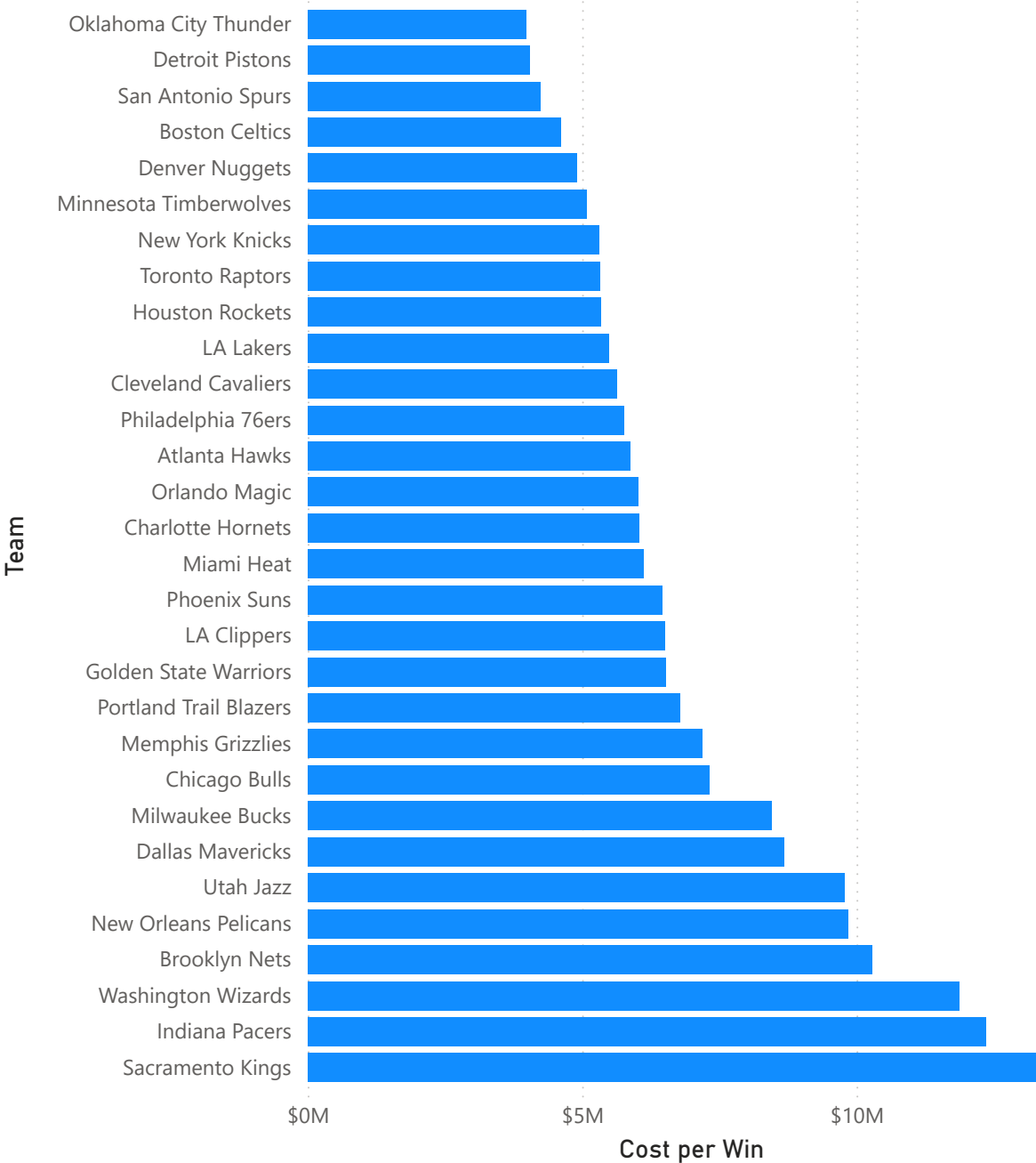
Cost per Win by Team
